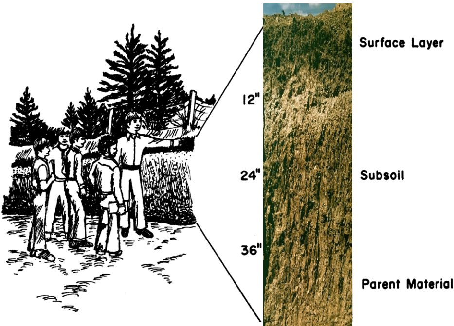
Figure 1. A soil profile.
